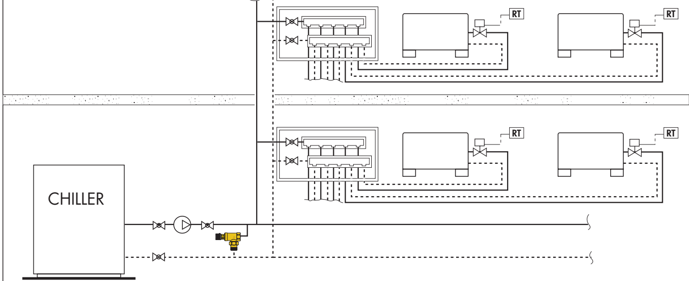
Chilled water system, central by-pass
