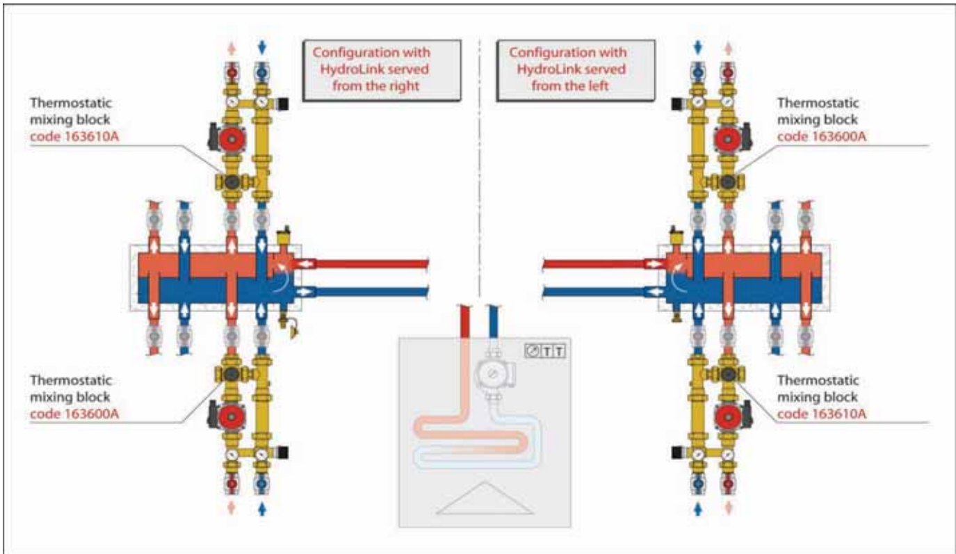
Diagram with 559 series HydroLink
